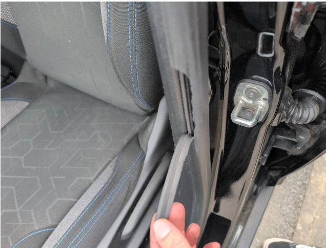
Photo 26 — Body seals
