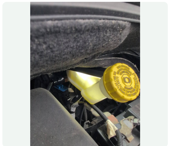
Photo 6 — Brake fluid
